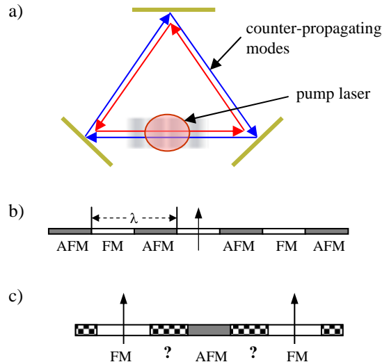
FIG. 2. (a) The ring cavity geometry, showing two degenerate, counter-propagating modes. The pump laser is taken to be oriented perpendicular to the plane of the figure, as shown. (b) Variation of the sign of the spin-spin potential due to a single Ising spin (the vertical arrow) in a ring cavity: spins in the white regions experience a ferromagnetic interaction with the pictured spin, whereas those in the grey regions experience an antiferromagnetic interaction. (c) Sign of the interaction experienced by a third spin due to two spins (the vertical arrows) positioned as shown in the figure. The two spins shown interact ferromagnetically and are therefore aligned; however, a third spin located in the patterned regions would be frustrated, as it would interact ferromagnetically with one of the depicted spins and antiferromagnetically with the other.
