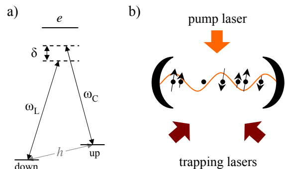
FIG. 1. (a) A possible atomic level structure for realizing associative memory models with XY spins. The detuning from two-photon resonance \delta is assumed to be much smaller than the detuning of both laser and cavity frequencies ( \omega_L and \omega_C respectively) from the atomic transitions. The microwave transition connecting the two spin states can be driven directly; such driving would correspond to the application of a magnetic field h . (b) Experimental setup. Atoms tightly trapped at fixed, random positions by the trapping lasers are pumped by a laser transverse to the cavity axis. The spins are ordered according to one of the patterns (i.e., a cavity mode profile, indicated by the wavy line) stored in the associative memory. Spins at even antinodes interact ferromagnetically with spins at other even antinodes, but antiferromagnetically with spins at odd antinodes. The interactions are strongest (weakest) for atoms located at antinodes (nodes); thus the spins of the atoms at the antinodes are more strongly organized, as depicted.
