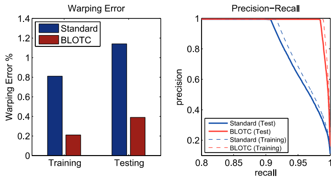
Figure 3. Comparison of standard and BLOT learning using the warping error metric on a 5.2 megapixel training set and a 1.2 megapixel testing set. The left plot shows warping error when classifier output is thresholded at 0.5, demonstrating a large relative reduction in error from standard to BLOT training. The right plot shows the precision-recall on outside voxel classification accuracy, which compensates for the class-imbalance. The warping error for all methods is provided in the supplementary material.
